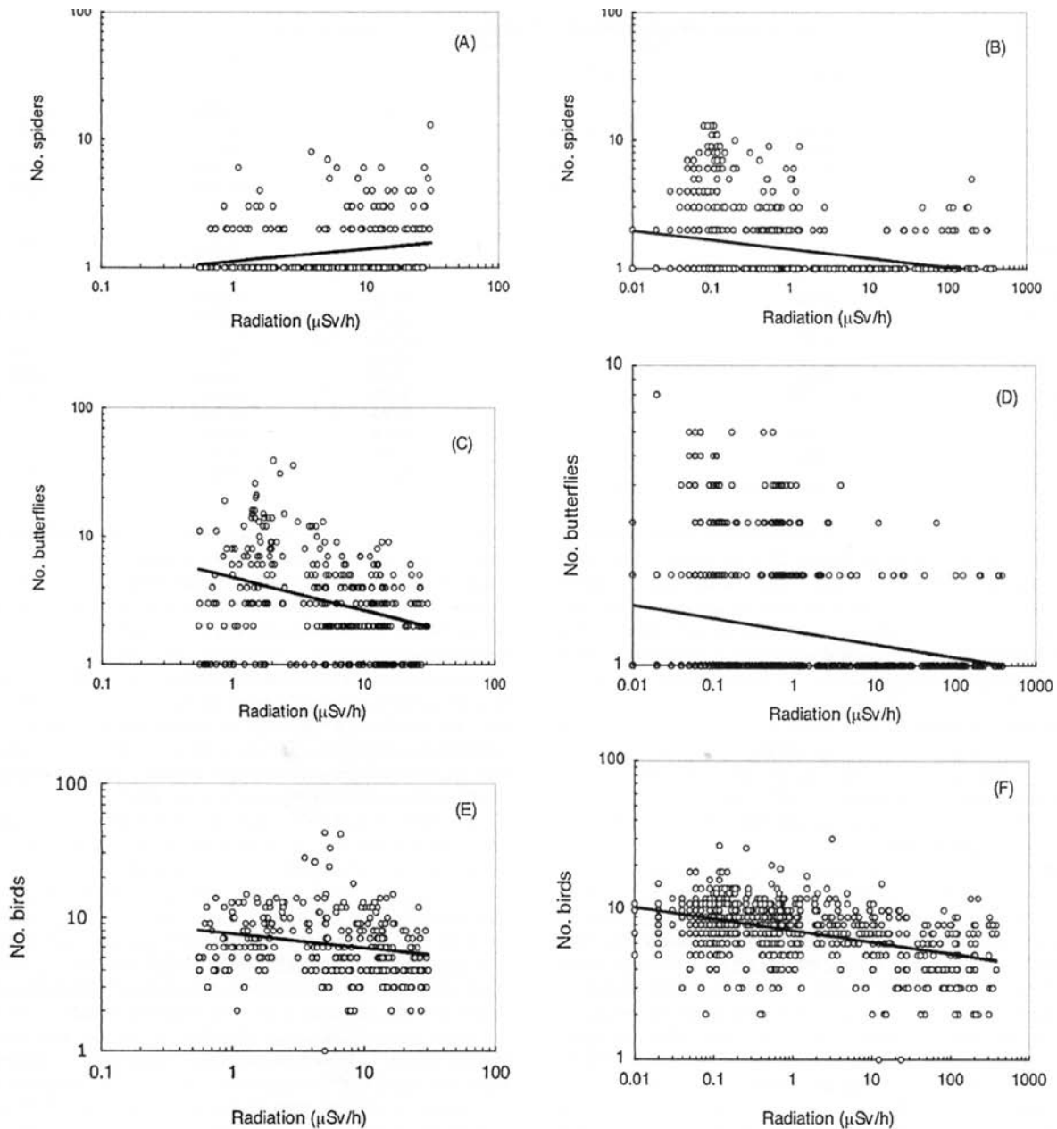
Fig. 3. Abundance of (A, B) spiders, (C, D) butterflies and (E, F) birds in relation to background radiation ( \mu\text{Sv/h} ) in Fukushima (A, C, E) and Chernobyl (B, D, F).
