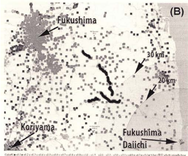
Fig. 1. Location of census areas around (A) Chernobyl, Ukraine and Belarus and (B) Fukushima, Japan. Census points in Fukushima are located in six areas. Note that levels of radiation in Fukushima have only been recorded at a limited number of sites.
