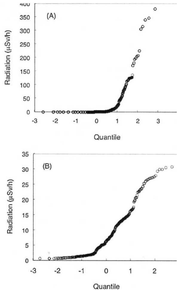
Fig. 2. Normal quantile plots of radiation levels (μSv/h) in (A) Chernobyl and (B) Fukushima.
